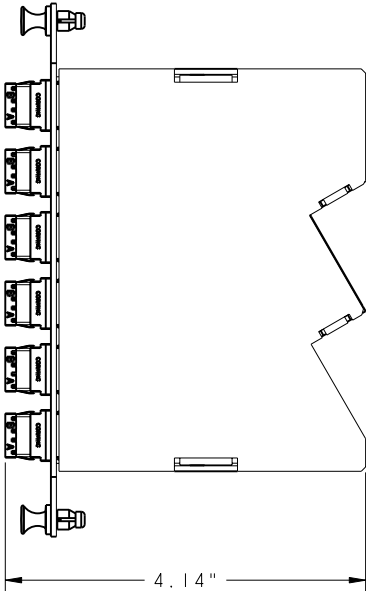
(Right view)
